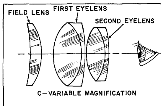
Figure 4-8. French, Plossl, and variable magnification eyepieces.
