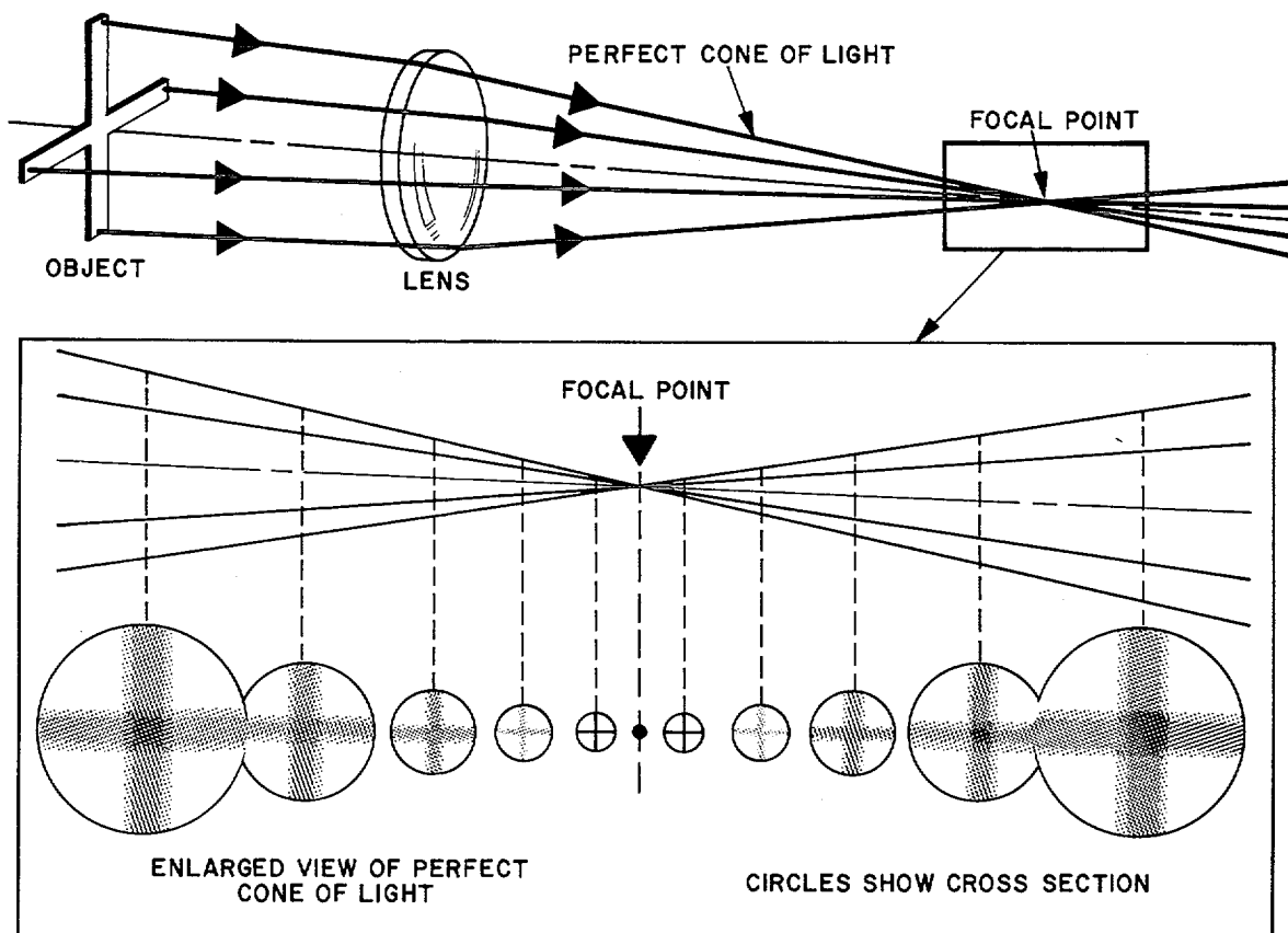
Figure 2-63. Proper refraction of light .
