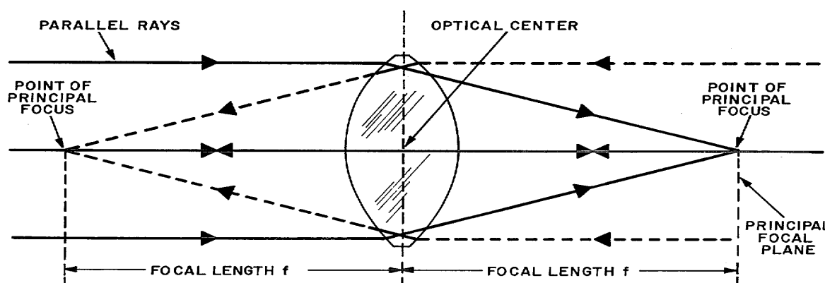
Figure 2-44. Focal lengths of convergent lens.
