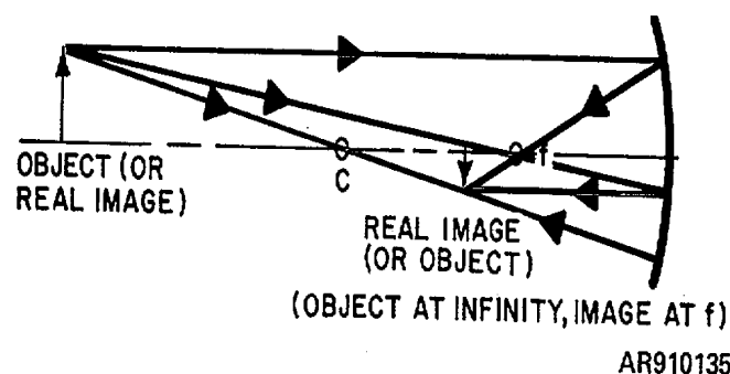
Figure 5-7. Concave mirror
