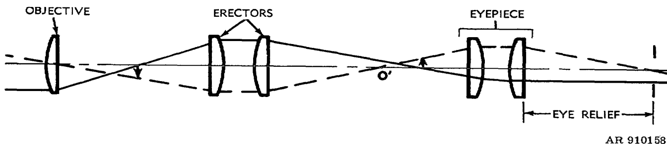
Figure 5-30. Eye relief-objective image outside erectors.
