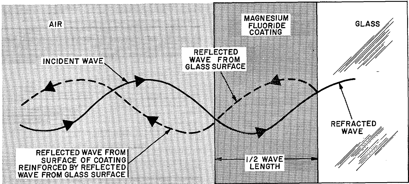
Figure 4-32. Light ray striking coated surface (coating one-half wave length in thickness).
