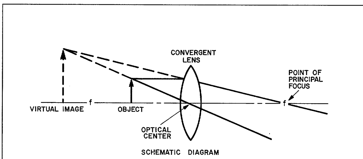
Figure 2-48. Magnification by reading glass-object within focal length.
