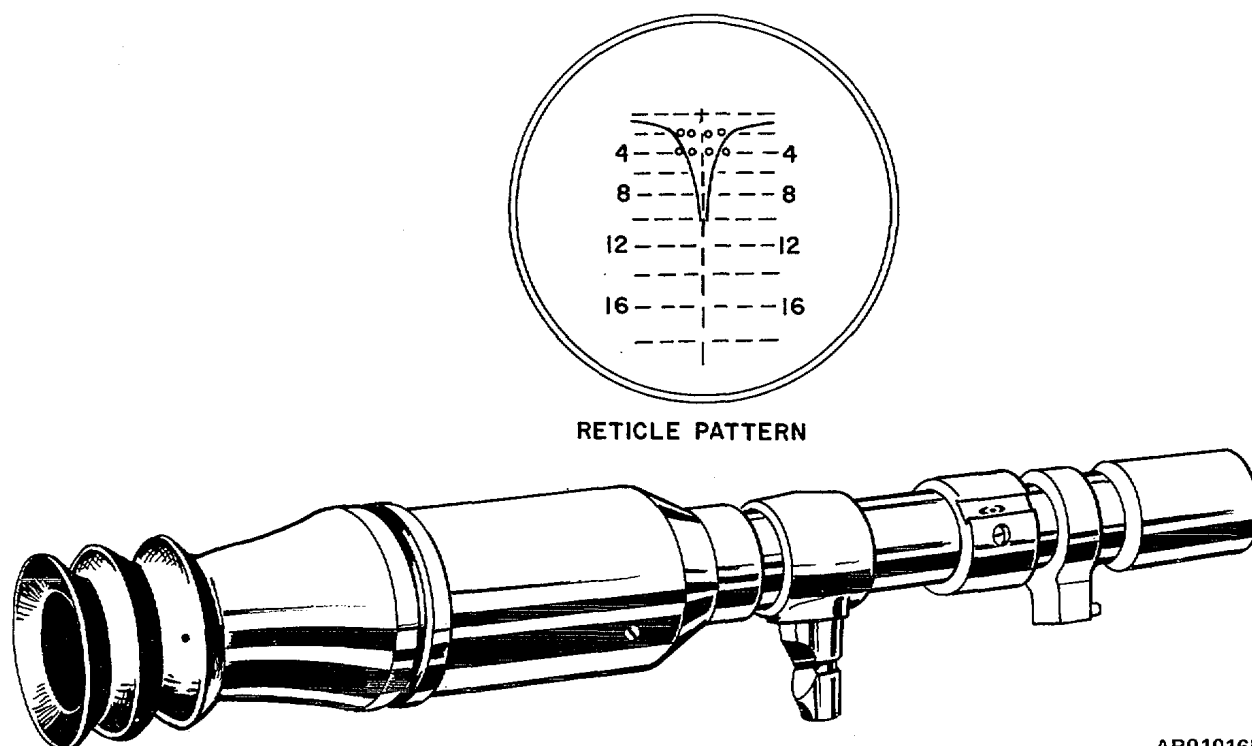
Figure 8-1. Telescope (Rifle)—assembled view, reticle pattern.
