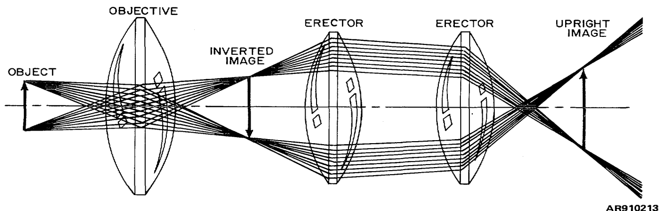
Figure B-13. Lens erecting system.
