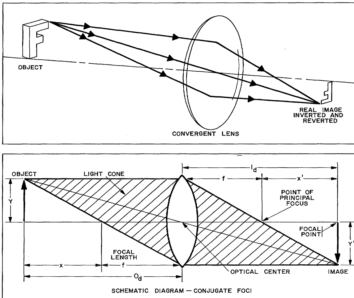
Figure 2-47. Image formed by convergent lens.
