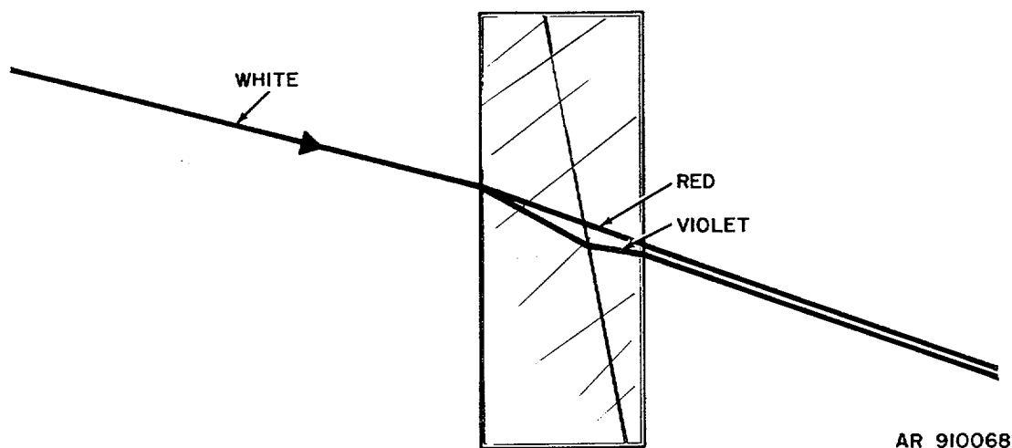
Figure 2-62. Correction of chromatic aberration of prisms.
