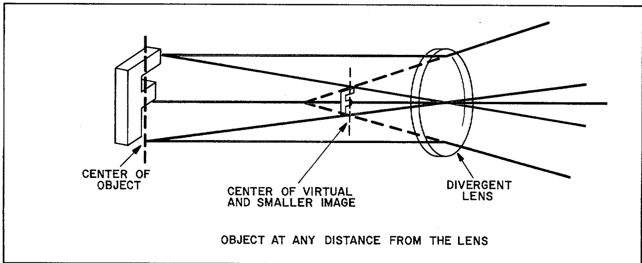
Figure 2-49. Effect of parallel rays on divergent lens.
