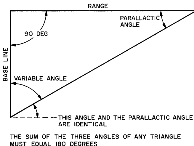
Figure 8-24. Fundamental triangle of range finder.
