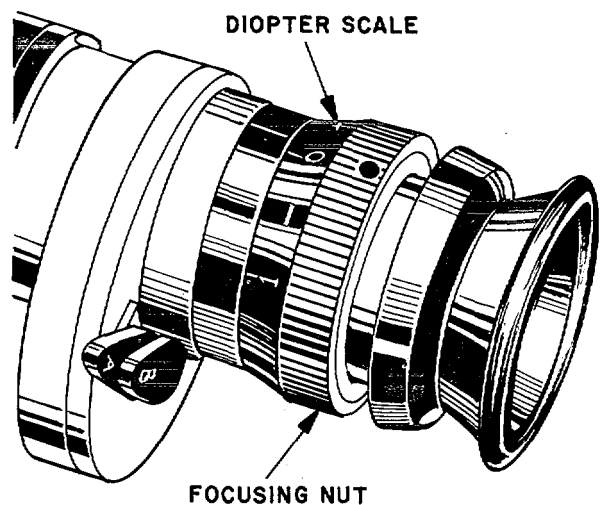
Figure 4-38. Diopter scale.
