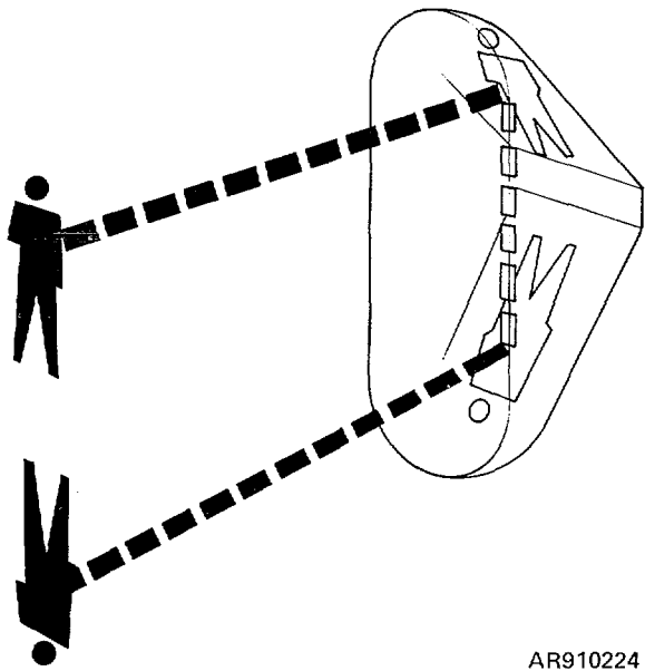
Figure B-24. Porro prism .
