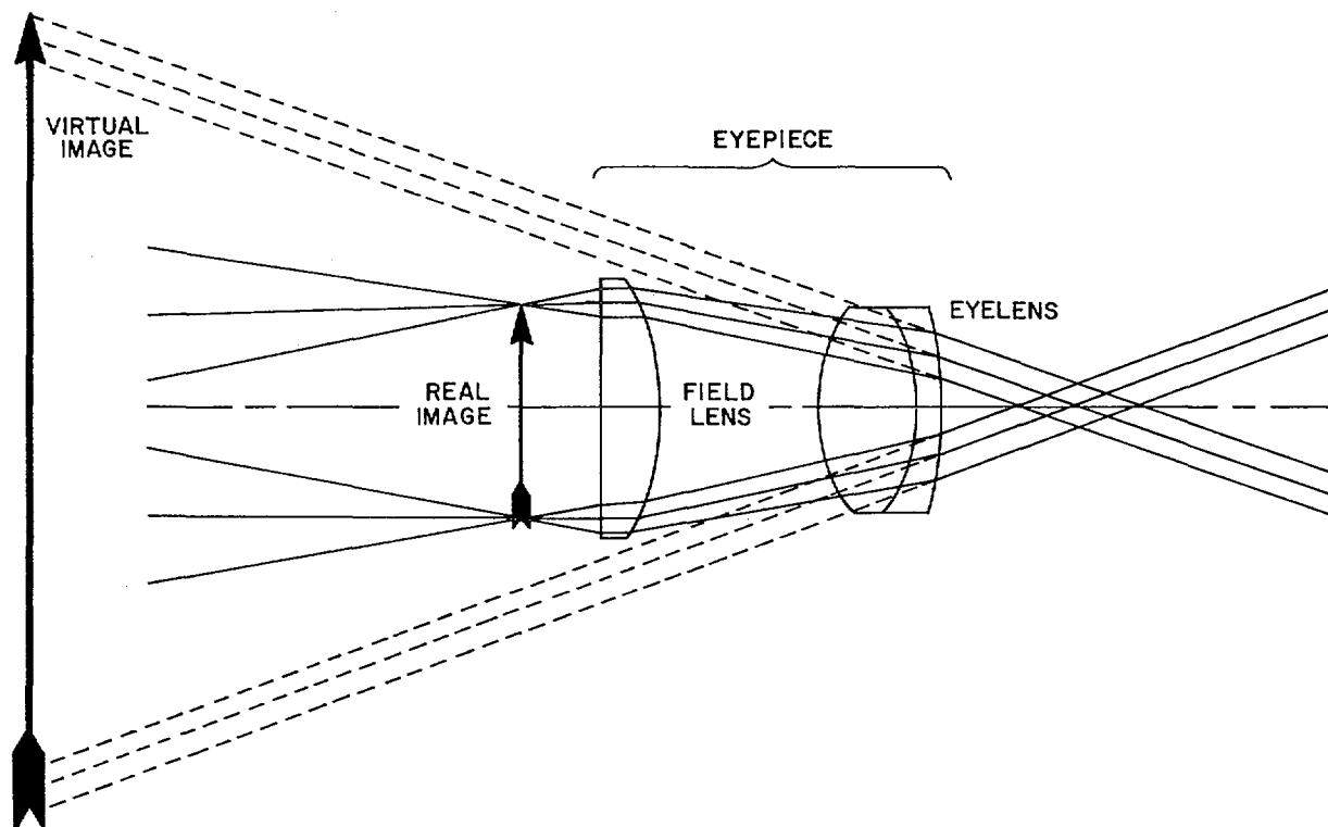
Figure B-14. Eyelens and fields lens of eyepiece.
