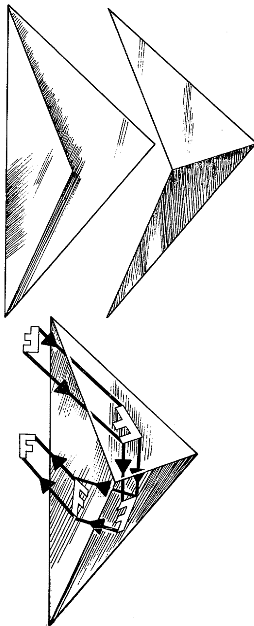
Figure 4-15. Triple mirror prism.
