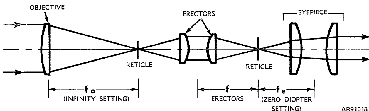
Figure 5-23. Reticle location
