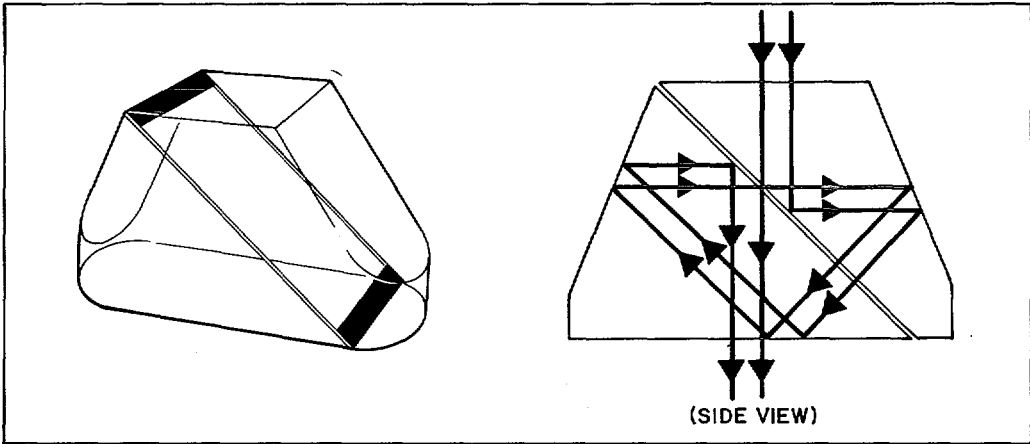
A-DOVE PRISM
