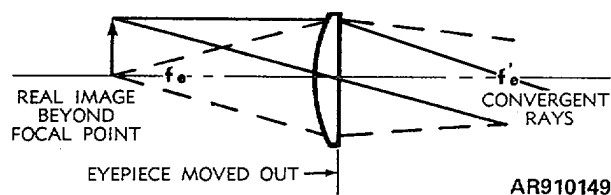
Figure 5-21. Plus setting for farsighted eye.
