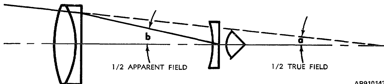
Figure 5-15. Objective diameter limits field in Galilean system
