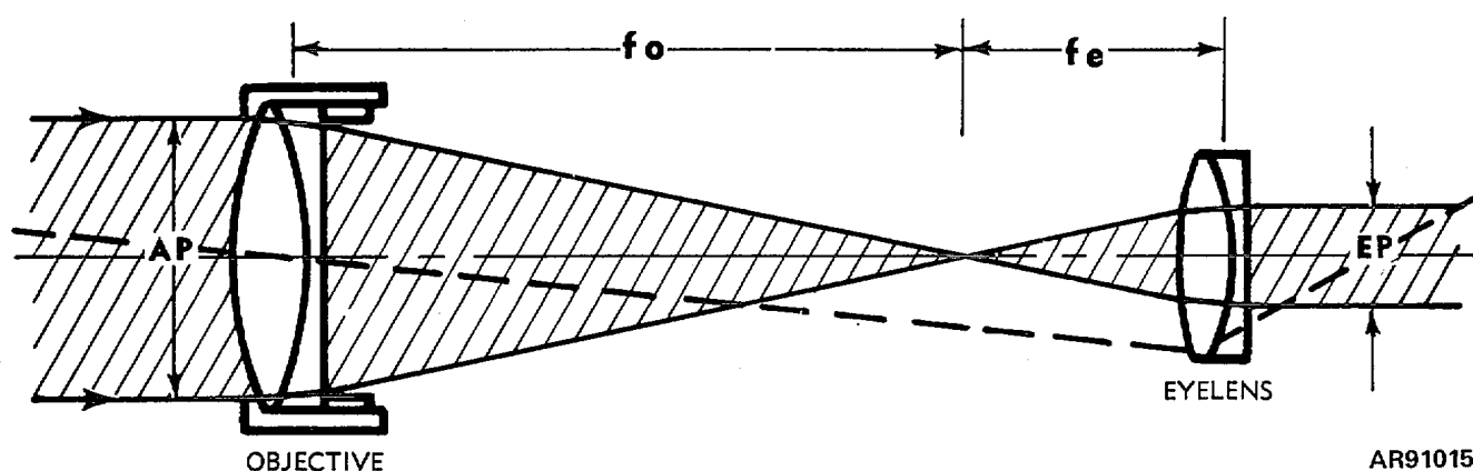
Figure 5-24. Entrance and exit pupils.
