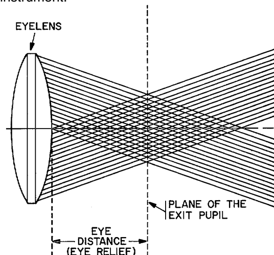
Figure 2-55. Eye distance.
