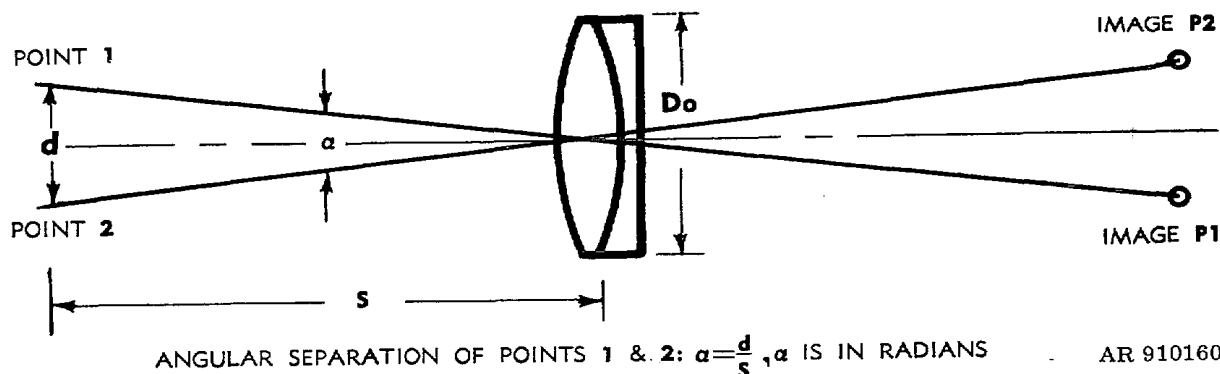
Figure 5-32. Angular limit of resolution.
