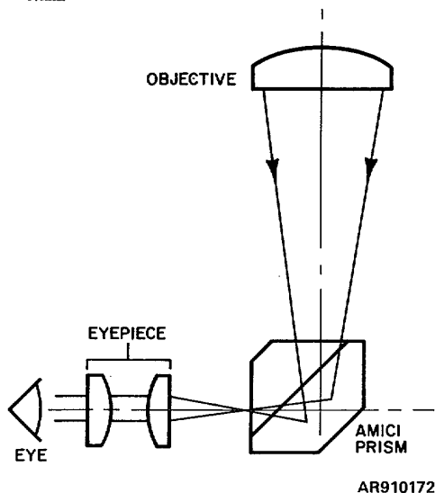
Figure 8-8. Schematic diagram of elbow telescope.
