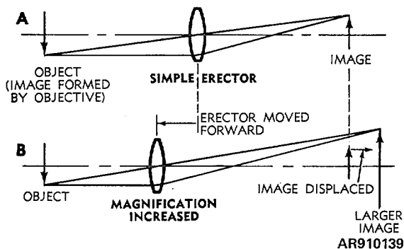
Figure 5-11. Simple erector.
