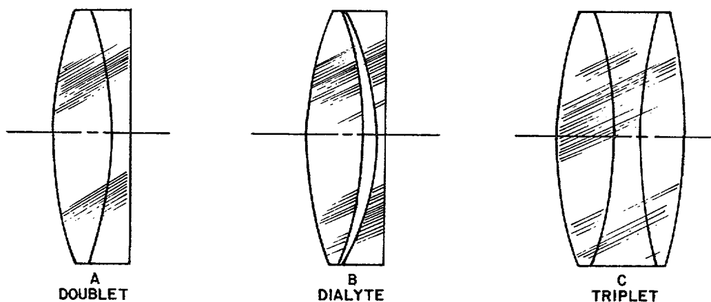
Figure 4-3. Types of objectives.
