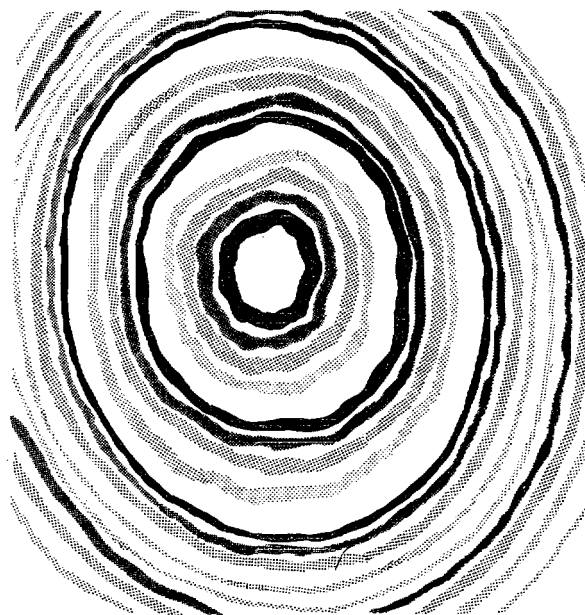
Figure 2-71. Newton's rings .
