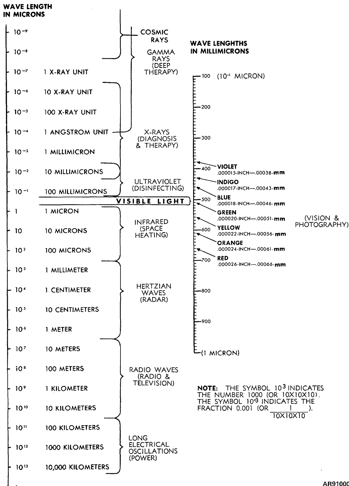
Figure 2-3. Electromagnetic spectrum.
