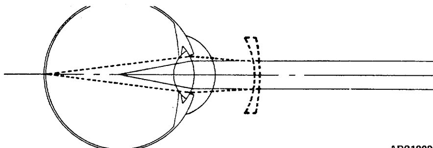
Figure 3-10. Nearsightedness (myopia)
