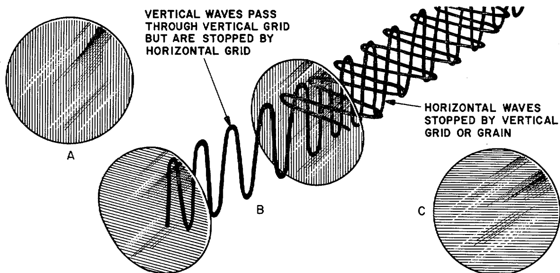
Figure 4-28. Principles of polarization of light.
