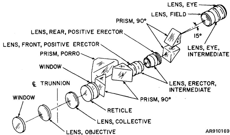
Figure 8-5. Articulated telescope - optical system diagram.
