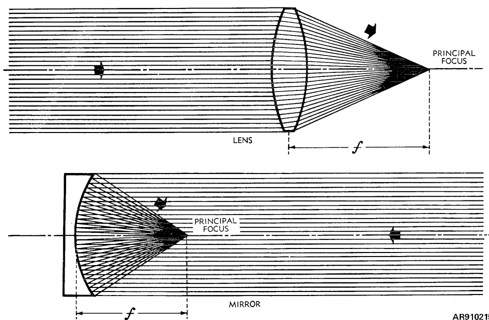
Figure B-15. Focal length of lens and mirror.
