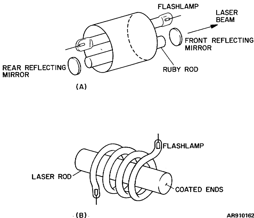
Figure 6-2. Solid-state rod lasers.
