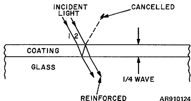
Figure 4-34. Low-reflectance coating.
