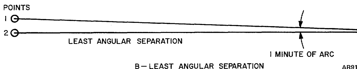
Figure 3-12. Visual Limitations
