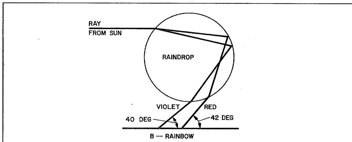
Figure 2-51. Dispersion.
