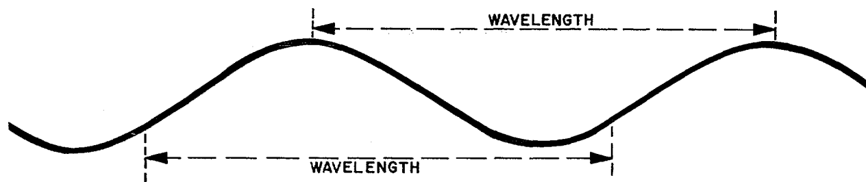
Figure 2-9. Wavelength
