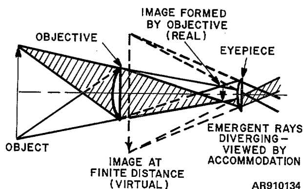
Figure 5-6. Refracting astronomical telescope
