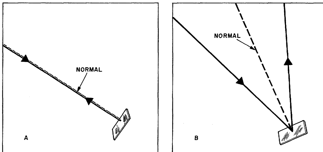
Figure 2-12. Beam of light reflecting back.
