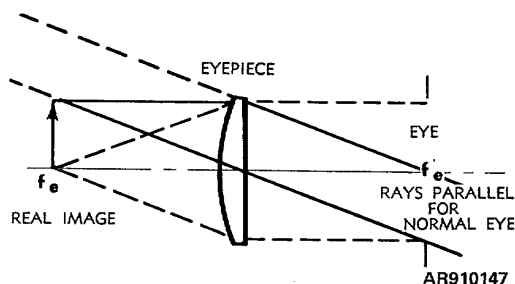
Figure 5-19. Zero diopter setting.
