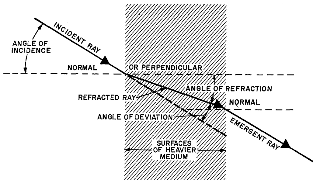
Figure 2-24. Terms used with reference to refracted light.
