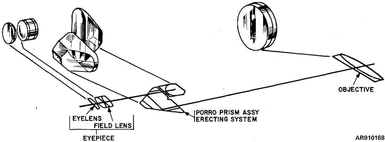
Figure 8-4. Observation telescope-optical elements and optical diagram.
