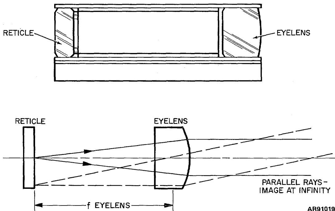
Figure 8-27. Collimator sight-optical system and optical diagram
