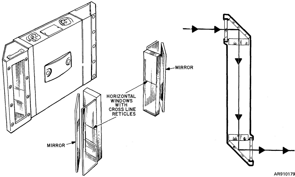
Figure 8-15. Periscope (Tank Observation)- assembled view, optical elements, and diagram of principle of operation.
