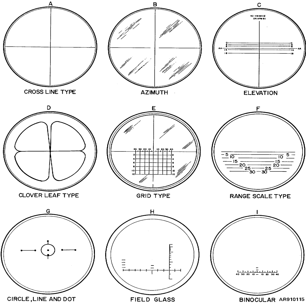
Figure 4-25. Representative types of reticle patterns.
