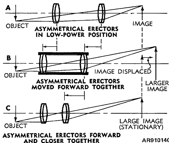
Figure 5-12. Asymmetrical erectors.
