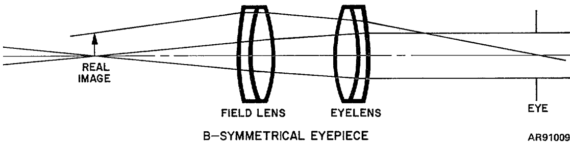
Figure 4-6. Huygenian and symmetrical eyepieces
