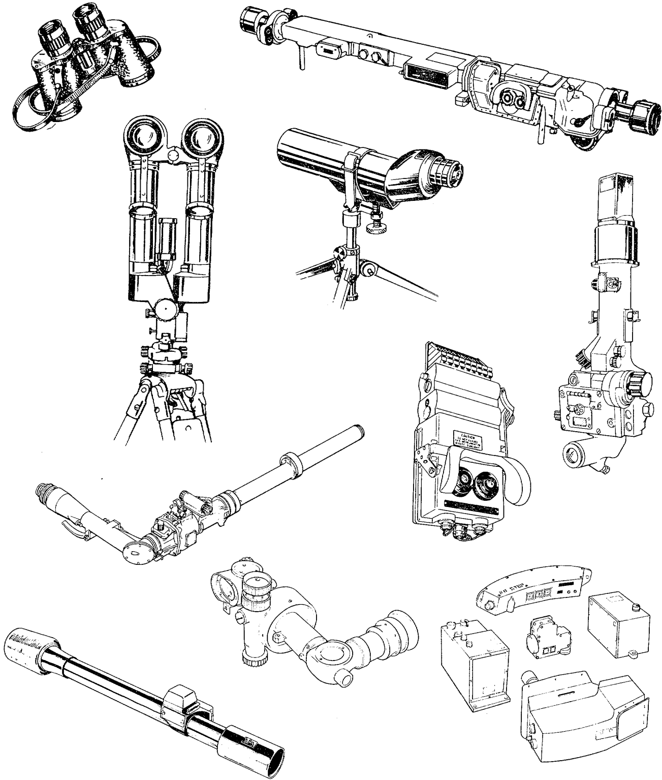
Figure 1-1. Military application of optics.
