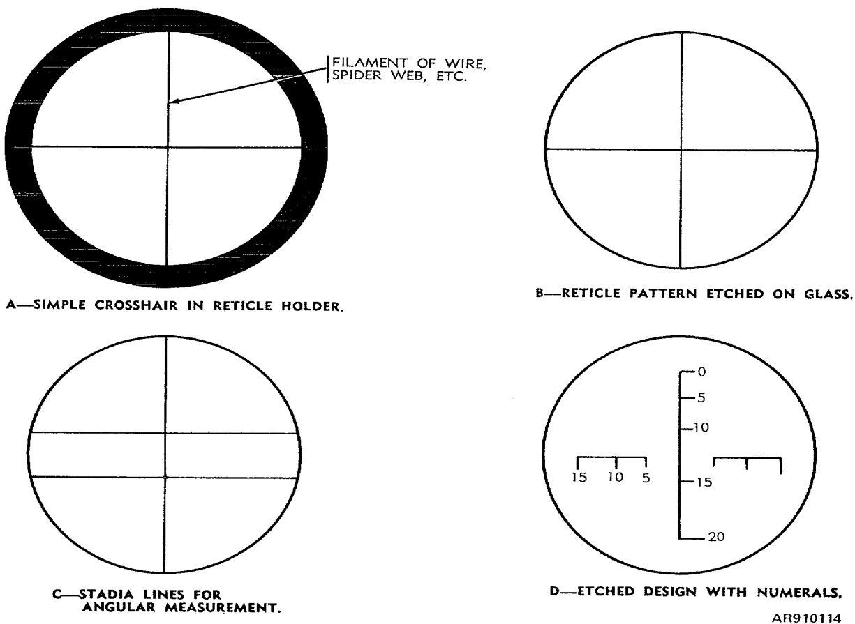
Figure 4-24. Representative types of reticles
