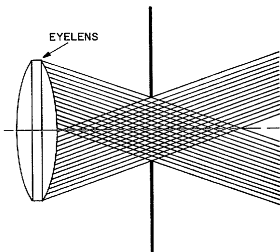
Figure 2-54. Exit pupil.
