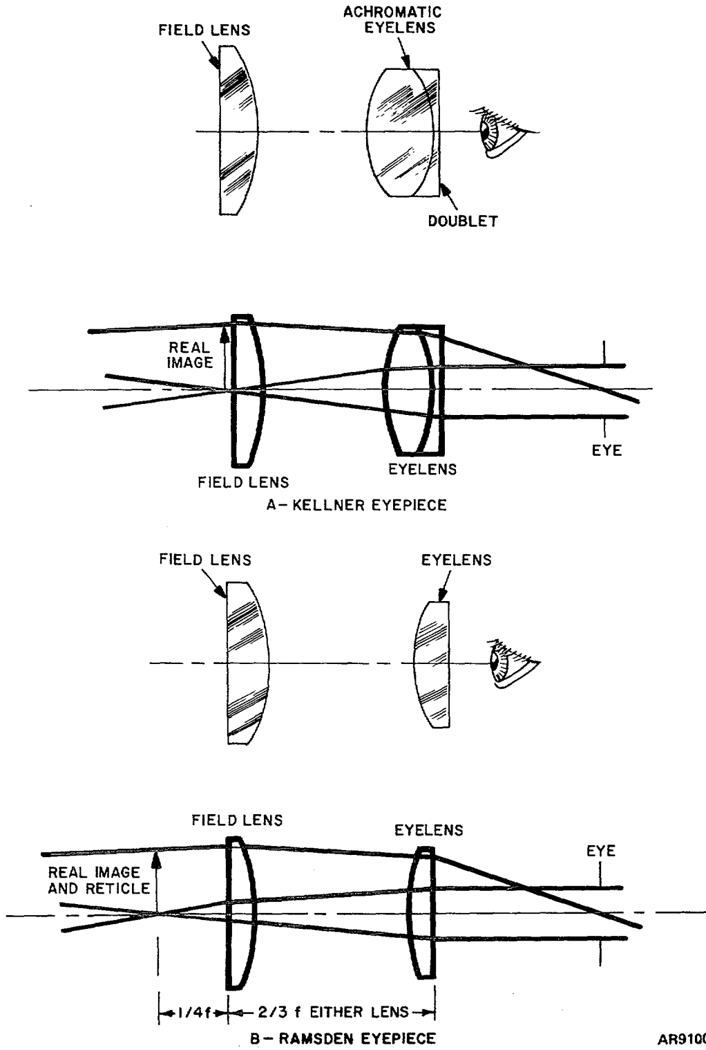
Figure 4-5. Kellner and Ramsden eyepieces.
