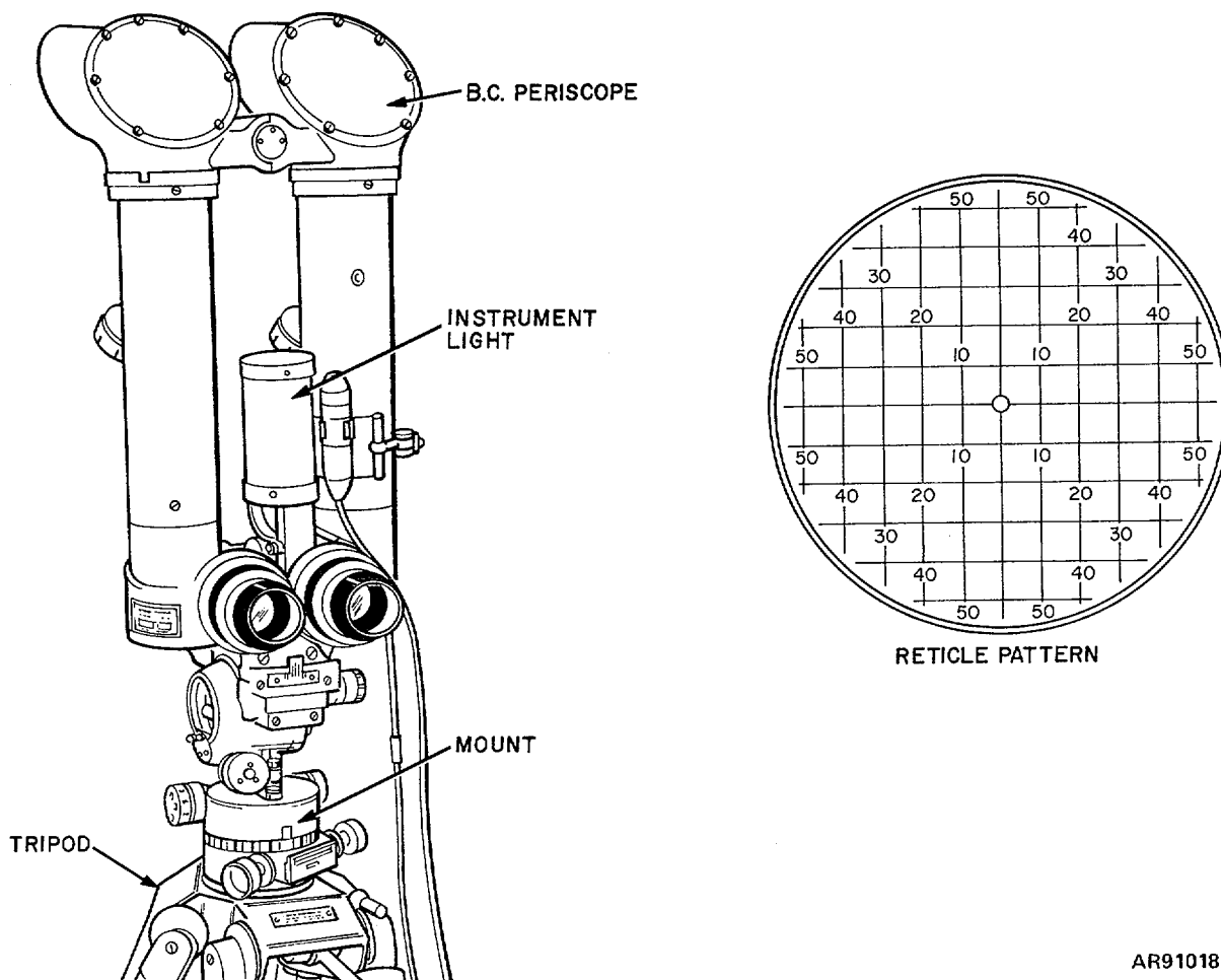
Figure 8-22. Battery commander's periscope - assembled view, reticle pattern.
