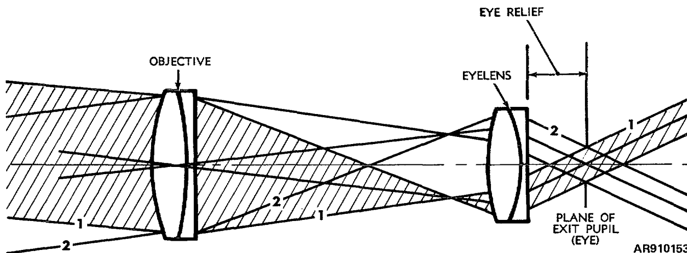
Figure 5-25. Exit pupil-virtual image of objective.
