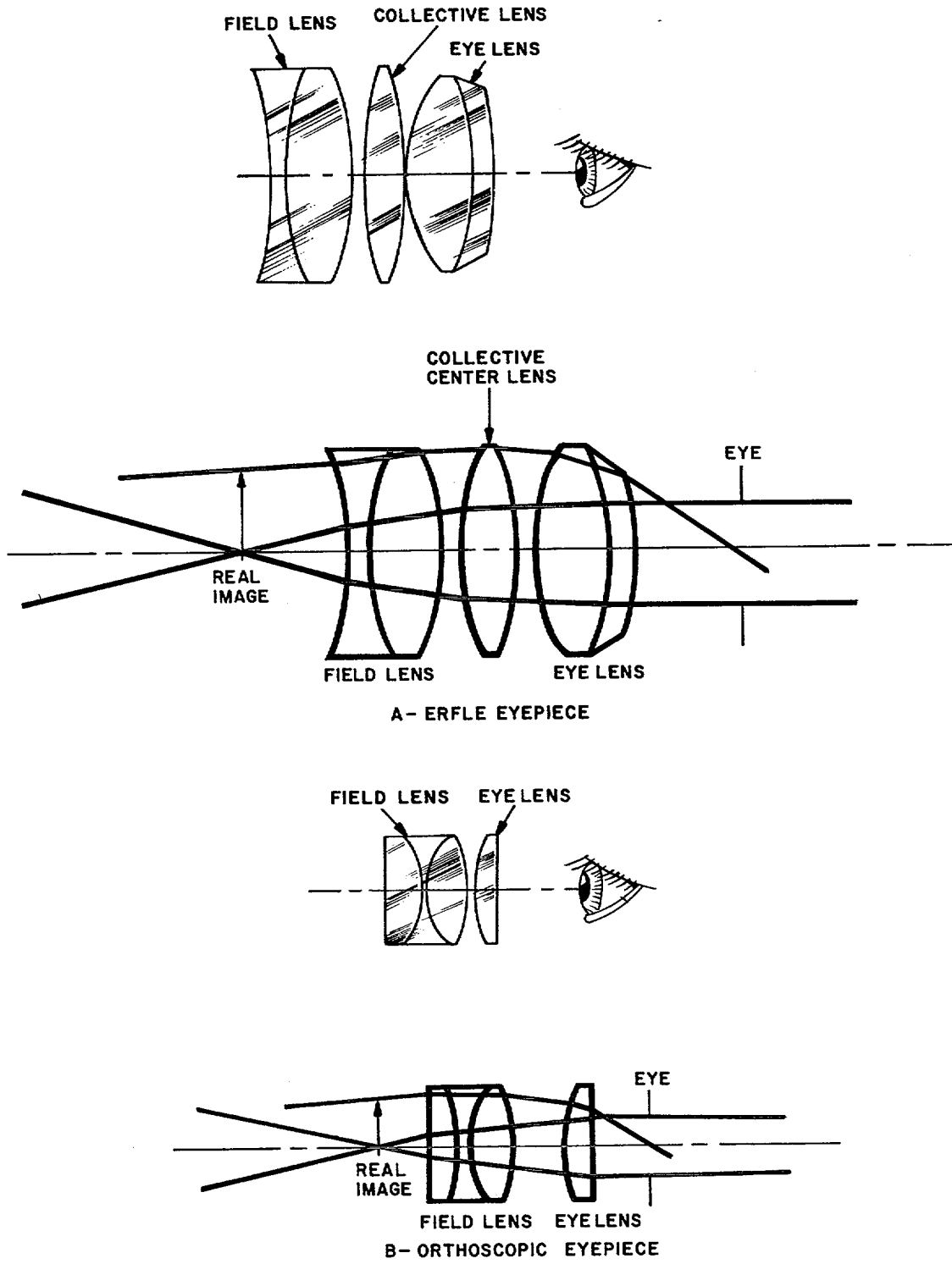
Figure 4-7. Erfle and orthoscopic eyepieces.
