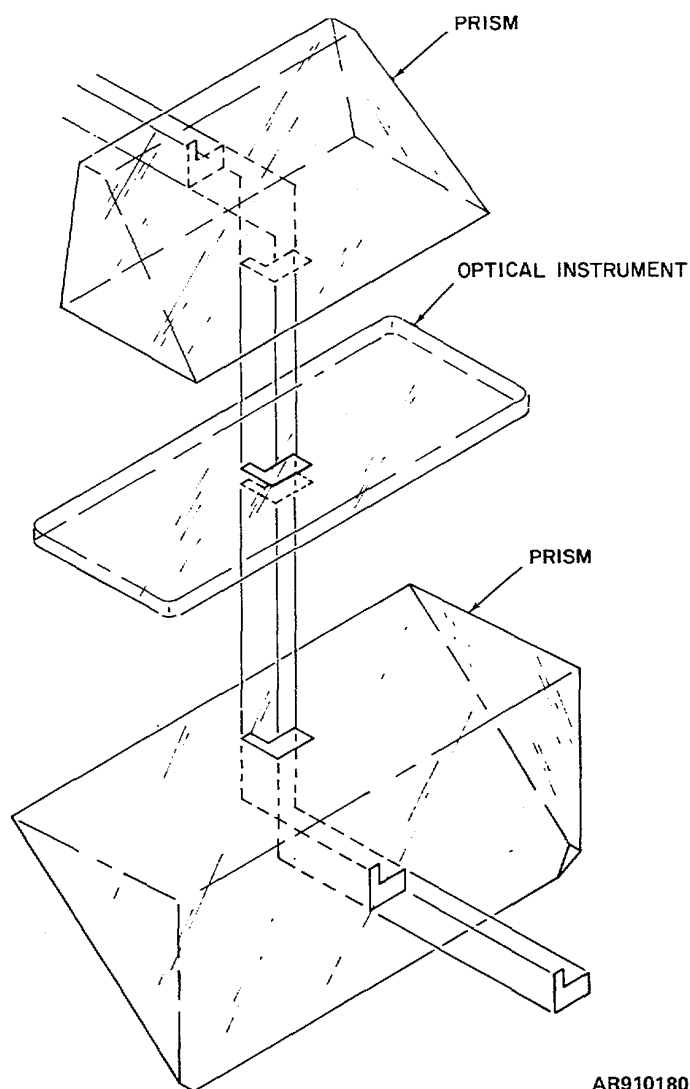
Figure 8-16. Optical diagram and optical elements of periscope.
