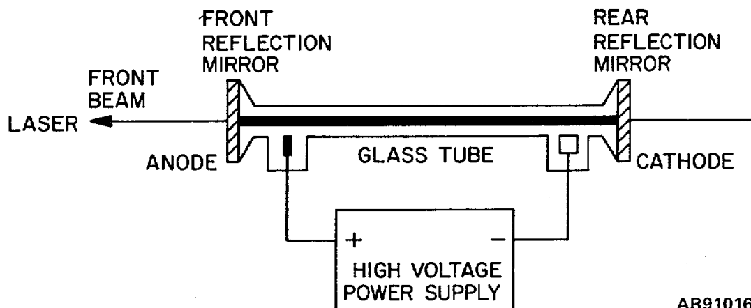
Figure 6-1. Gas laser.
