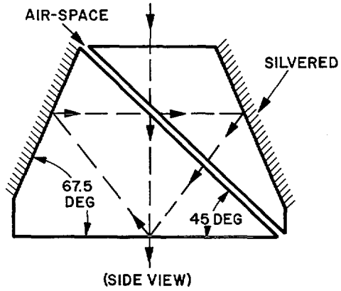
B-PECHAN PRISM
