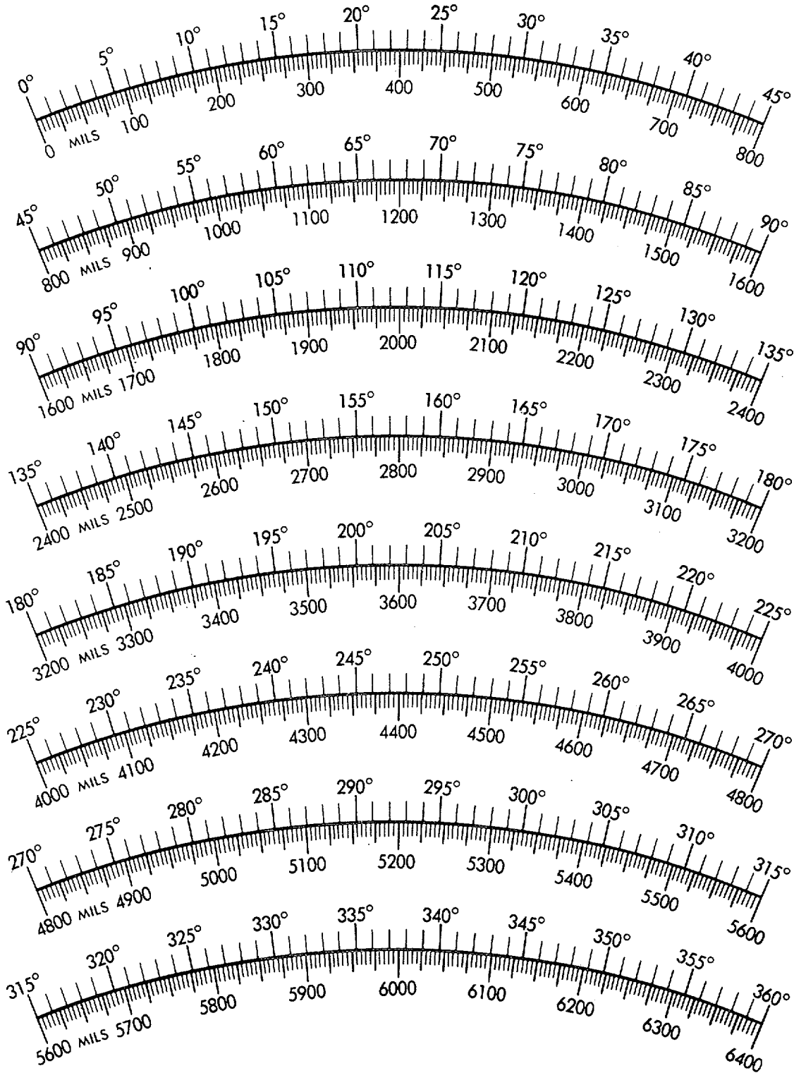
Figure 10-1. Artillery mil-degree conversion chart.
