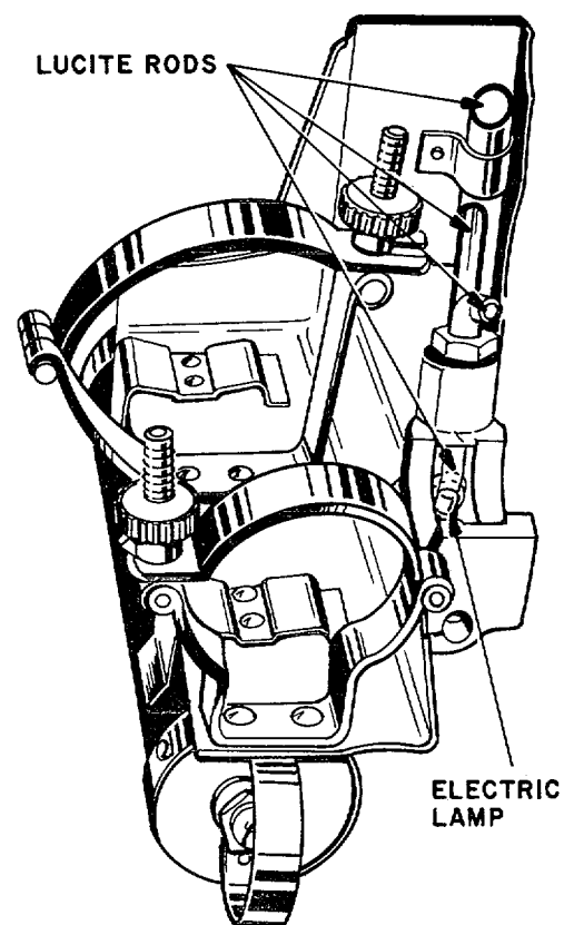
Figure 4-29. Instrument light for panoramic telescope.
