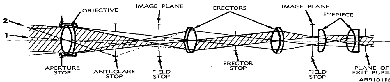
Figure 4-26. Diaphragm (stop) location.
