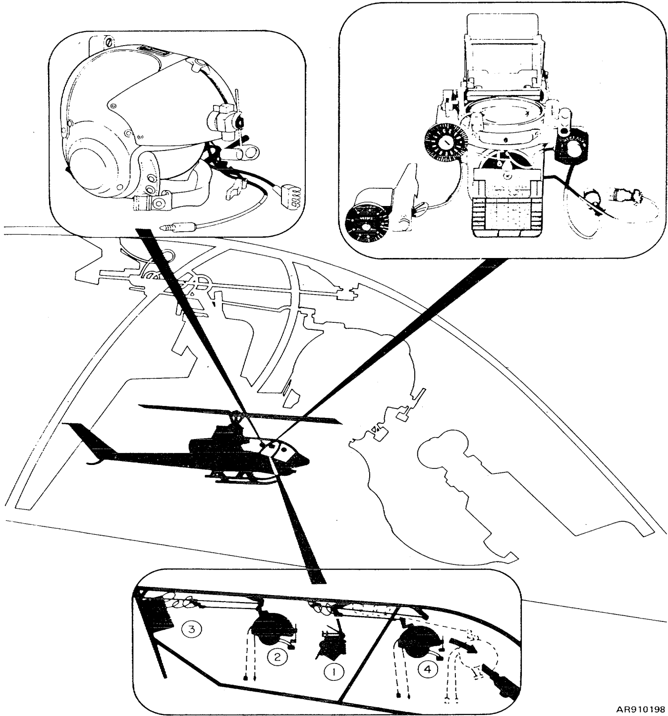
Figure 8-31. Fire control subsystem, helmet-directed.
