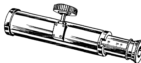
Figure 5-26. Ramsden dynameter.
