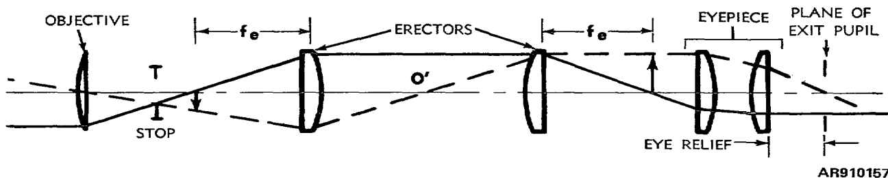
Figure 5-29. Eye relief-symmetrical erectors with real images at focal points of erectors and image O' of objective between erectors.
