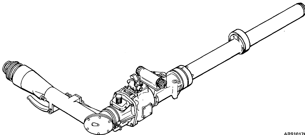
Figure 8-12. Elbow telescope ( Self Propelled Howitzer)- assembled view.
