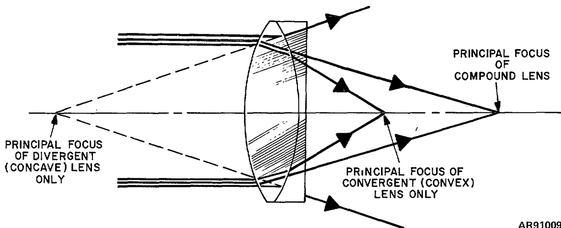
Figure 4-2. Comparative focal lengths of elements in compound lens.
