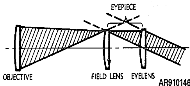
Figure 5-18. Function of field lens in eyepiece.
