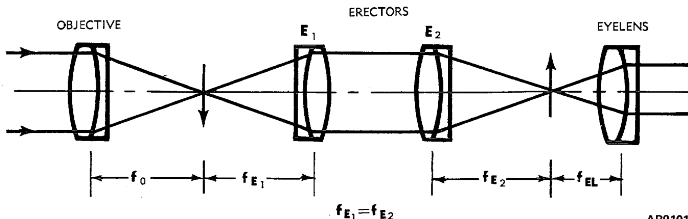
Figure 5-10. Symmetrical erectors.
