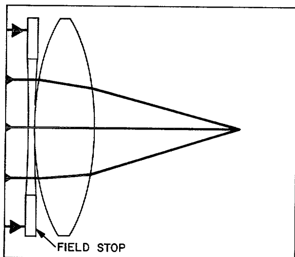
A — EFFECT OF FIELD STOP ON SPHERICAL ABERRATION
