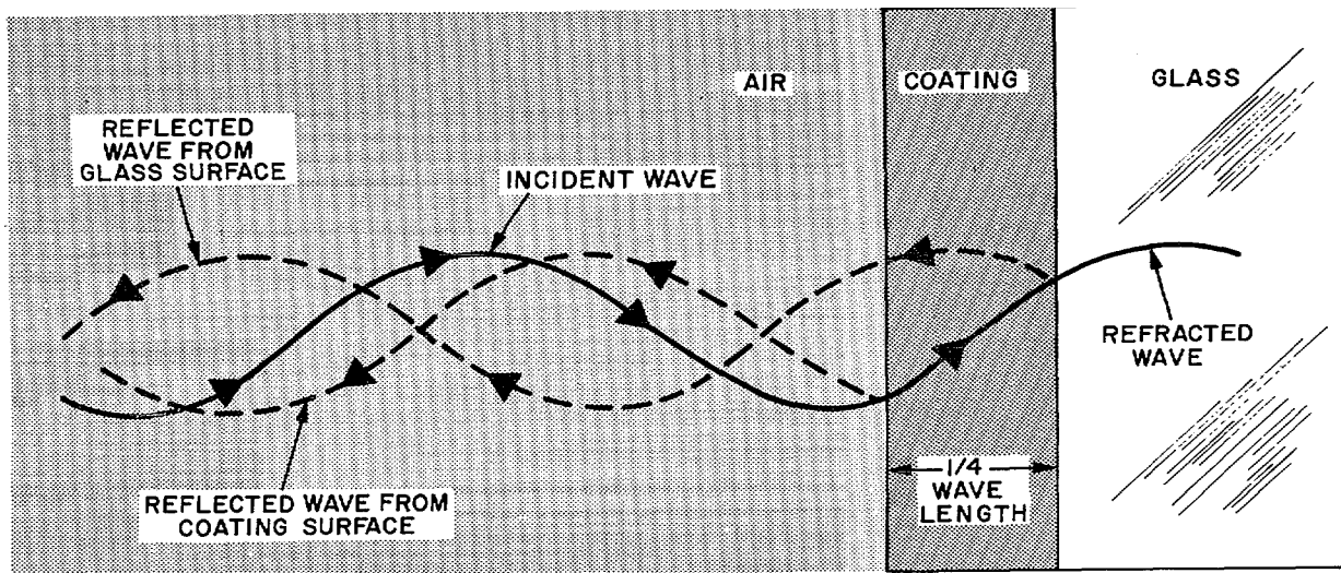
Figure 4-33. Light ray striking coated surface (coating one-quarter wavelength in thickness).
