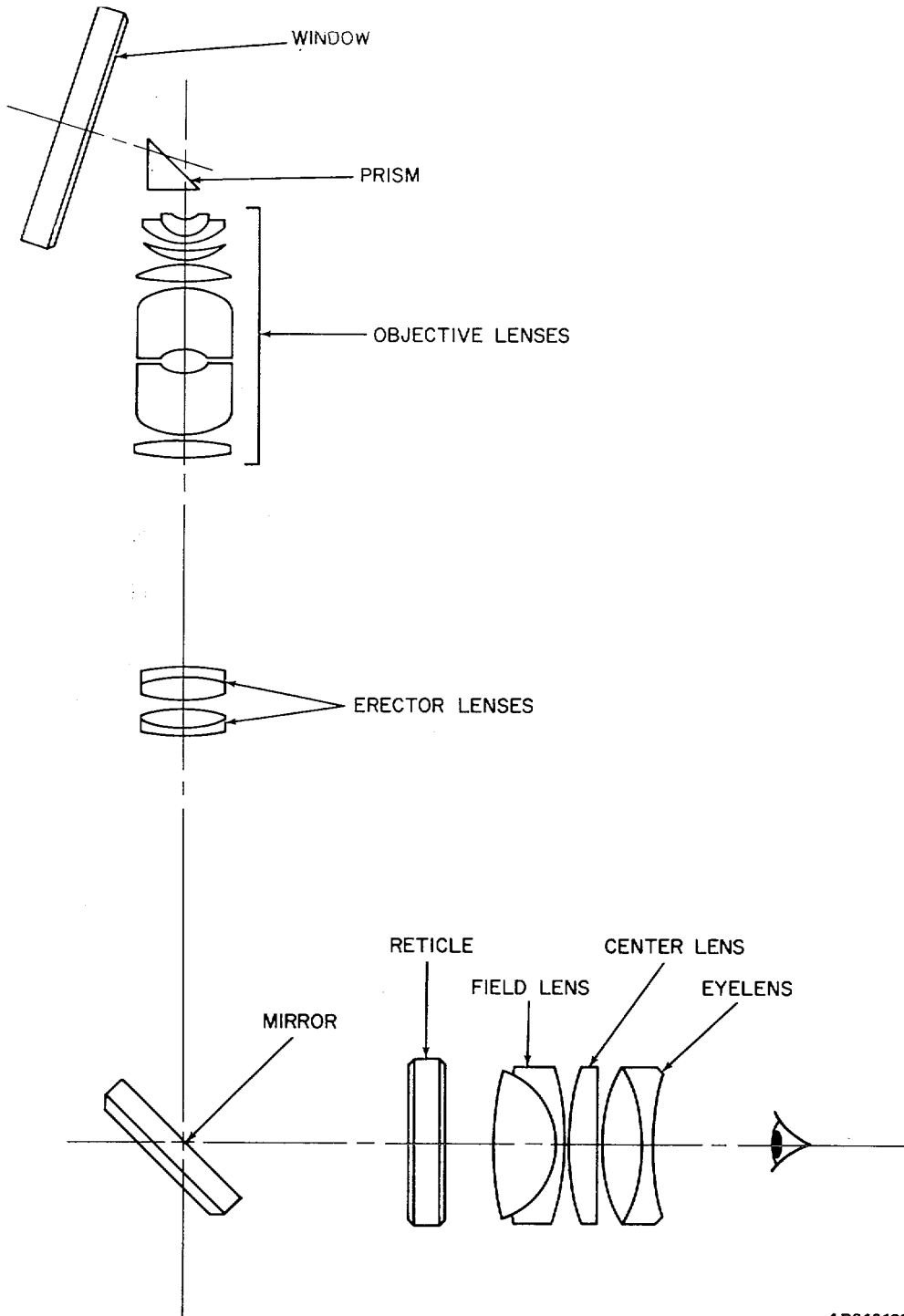
Figure 8-19. Periscope (Tank) - diagram of optical system.
