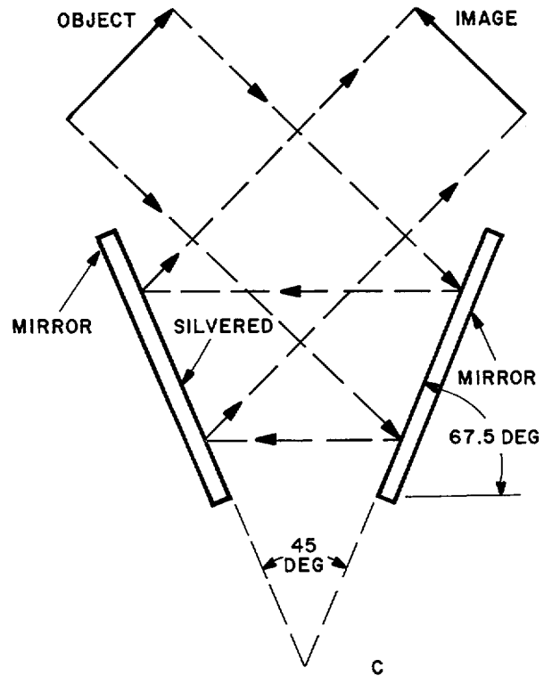
Figure 4-14. Pentaprism (diagrams show same effect obtained with mirrors).
