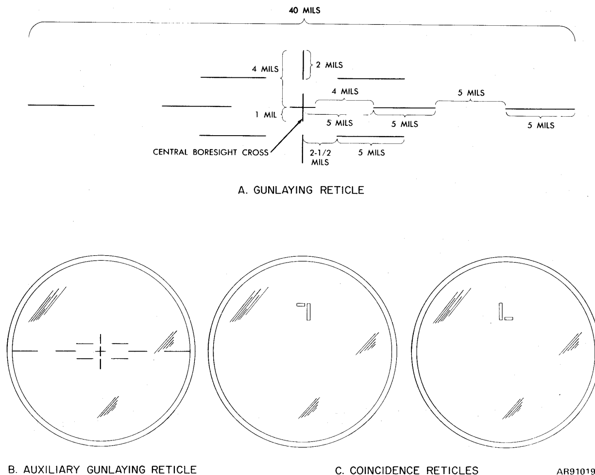
Figure 8-26. Range finder reticle patterns.
