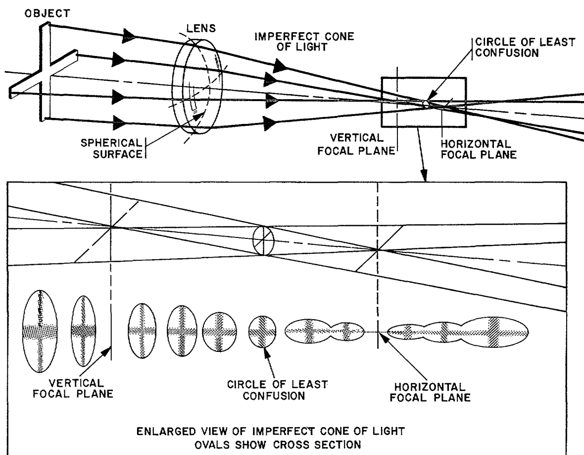
Figure 2-64. Astigmatic refraction of light .
