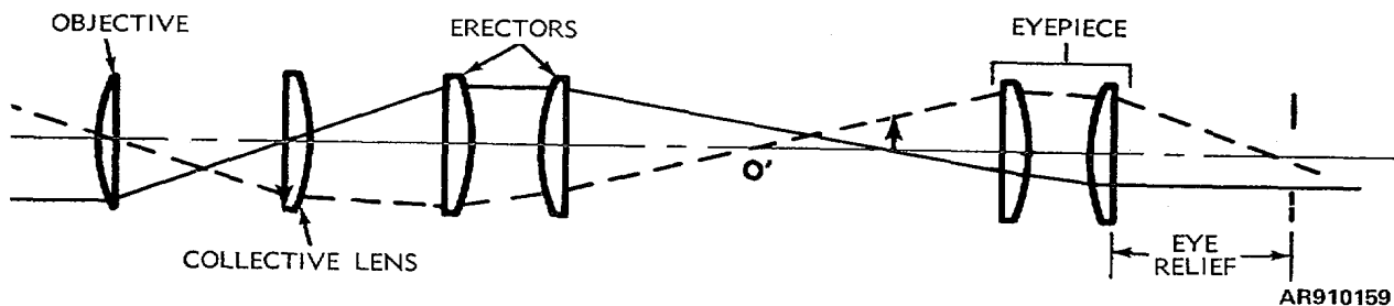
Figure 5-31. Eye relief-collective lens in system.
