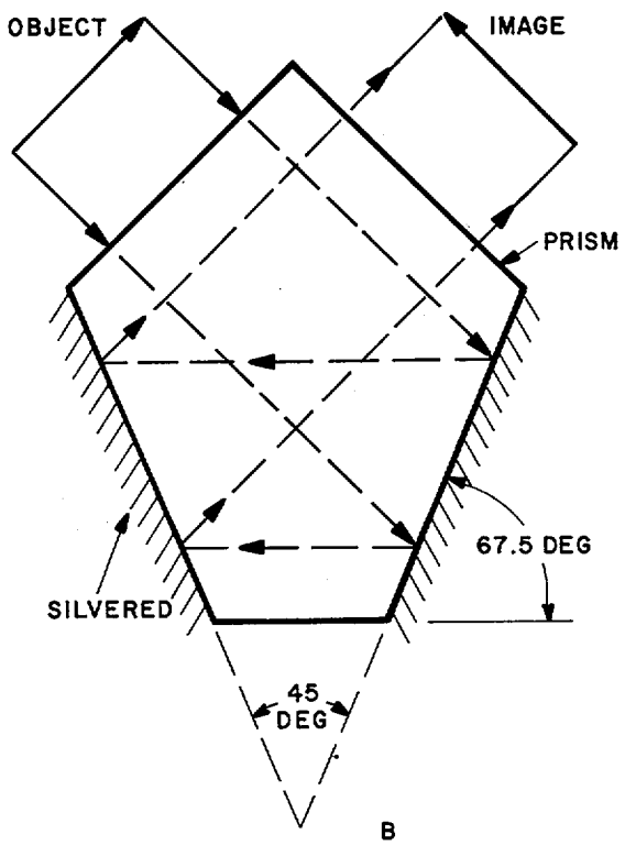
Figure 4-14. Pentaprism (diagrams show same effect obtained with mirrors).
