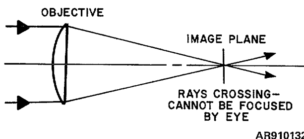
Figure 5-4. Objective lens.
