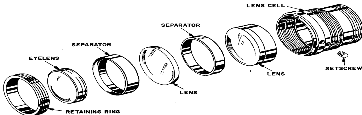
Figure 4-35. Lens cell, separators, lenses, and retaining ring.
