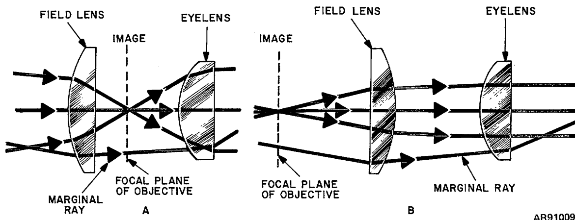
Figure 4-4. Typical light paths through field lens and eyelens of eyepieces.
