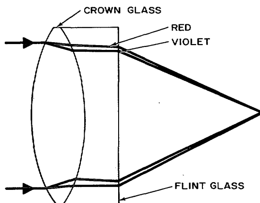
Figure 2-61. Correction of chromatic aberration of lens.
