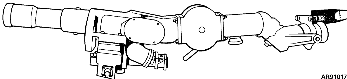
Figure 8-7. Articulated telescope ( Self-Propelled Vehicle)-assembled view.
