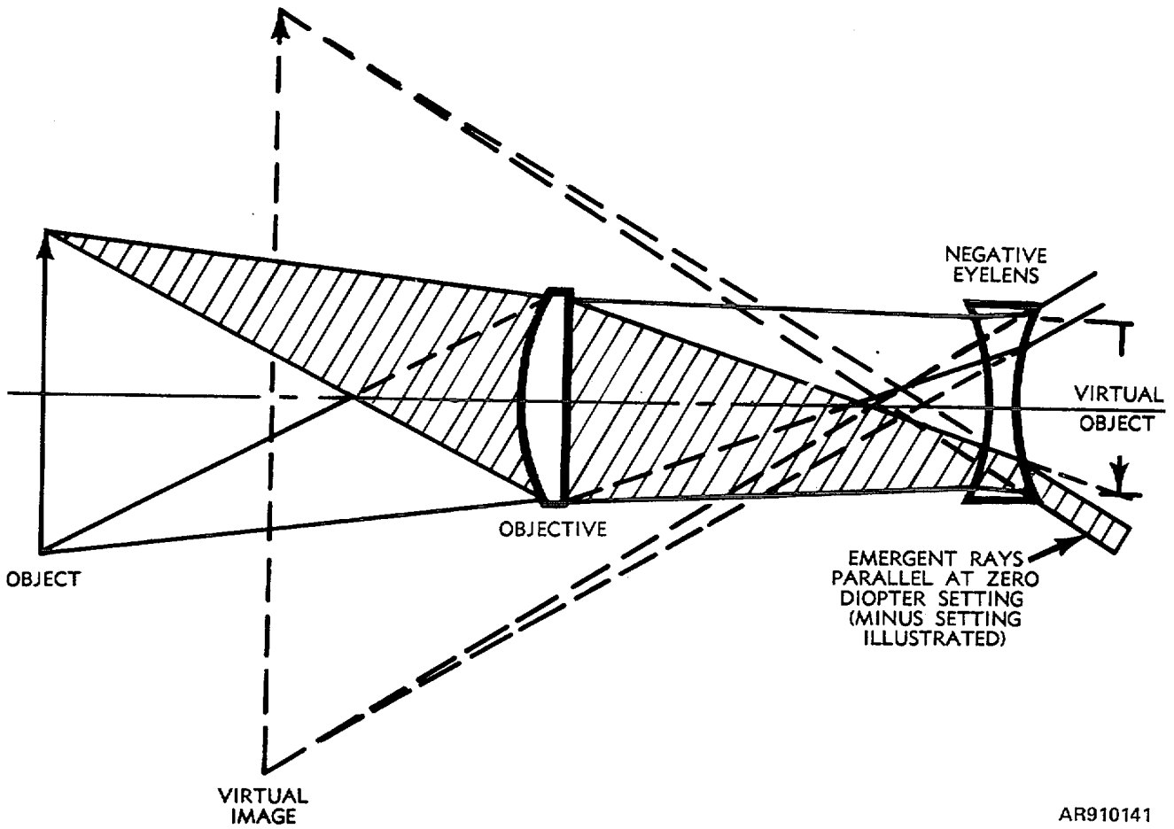
Figure 5-13. Galilean system.
