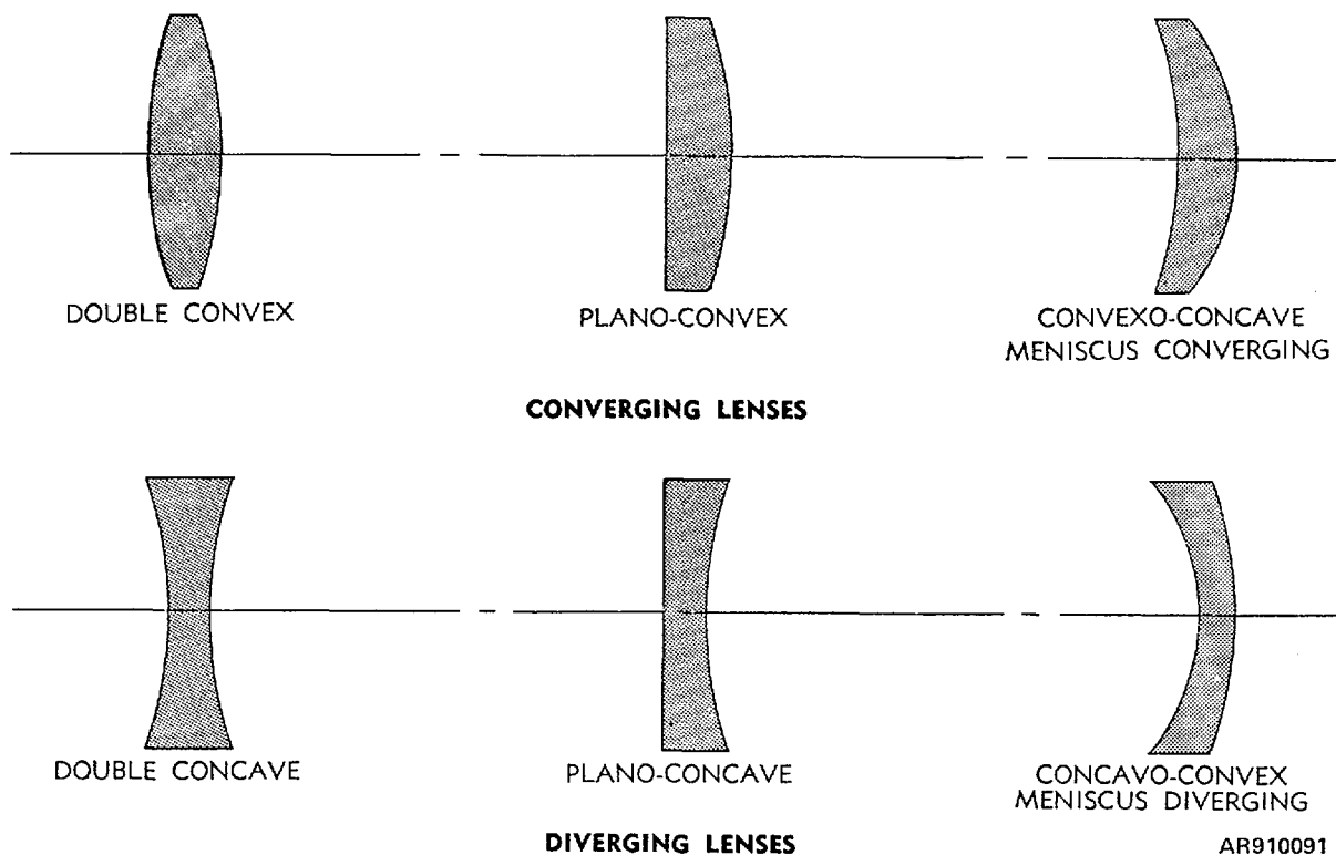
Figure 4-1. Types of simple lenses.
