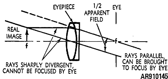
Figure 5-17. Function of eyepiece.
