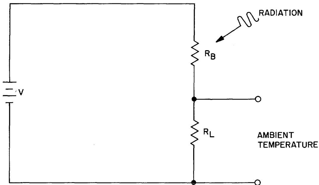
Figure 7-2. Bolometer circuit.
