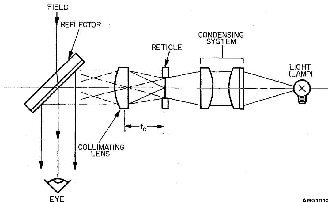
Figure 8-28. Reflex sight.
