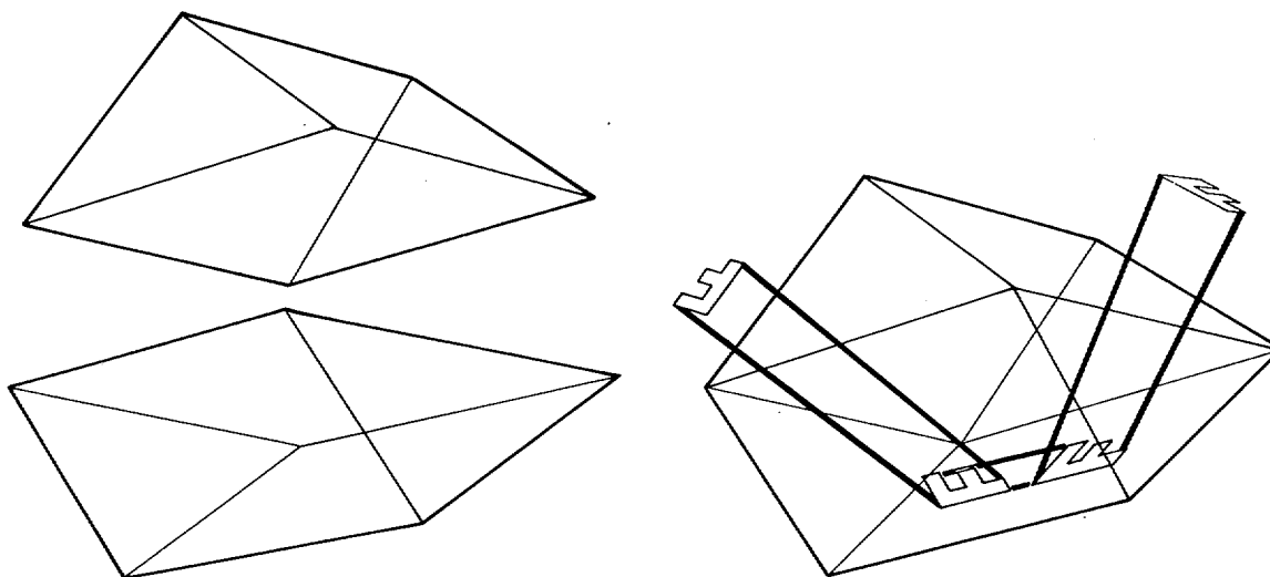
Figure 4-11. Amici or roof-angle prism.
