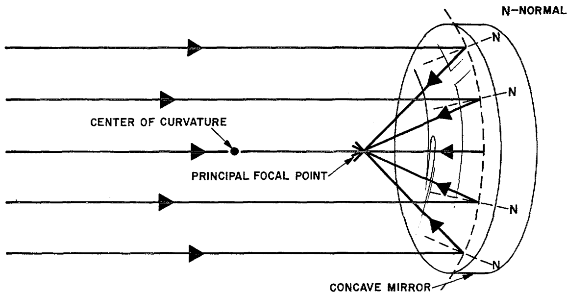
Figure 2-19. Reflection from concave mirror.
