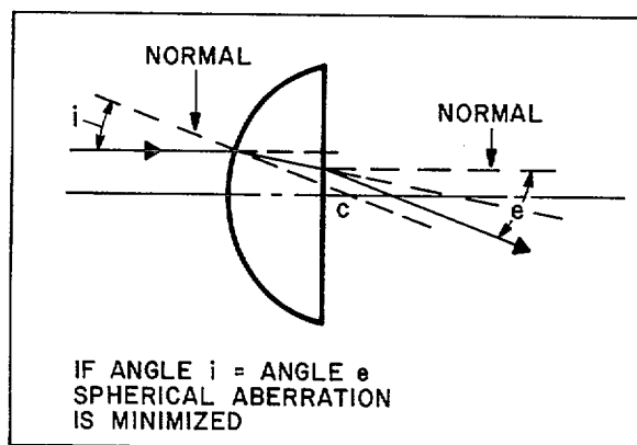
B — SPHERICAL ABERRATION — REDUCTION IN TELESCOPE
