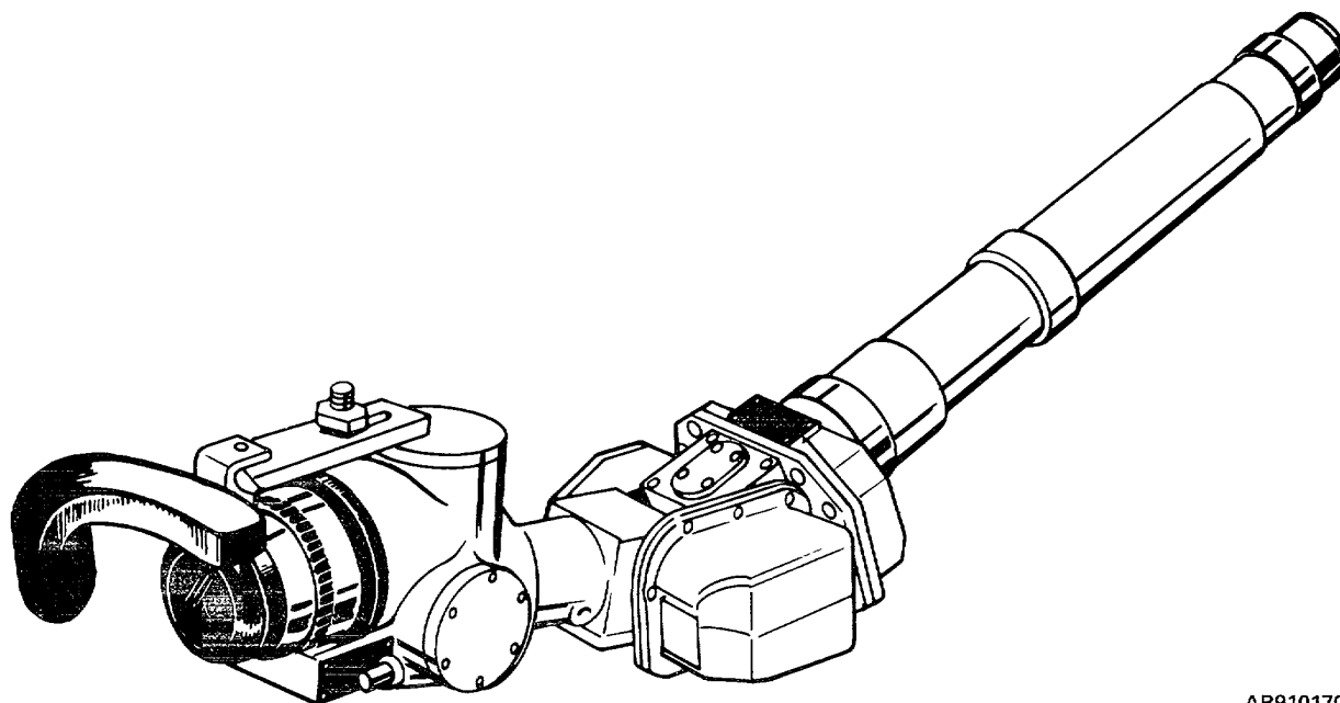
Figure 8-6. Articulated telescope (Tank) - assembled view.
