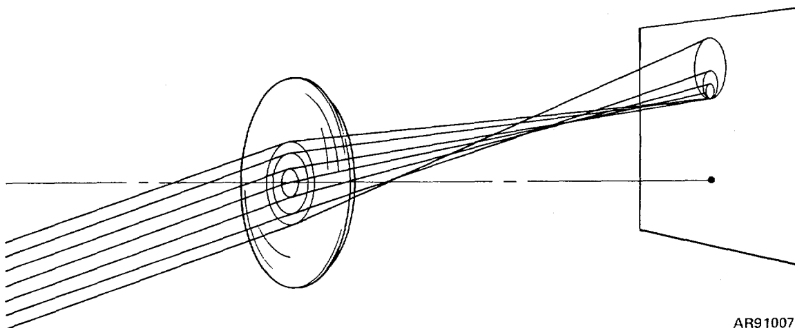
Figure 2-65. Coma
