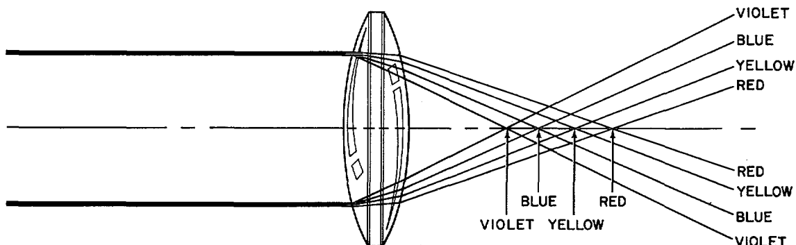
Figure 2-60. Chromatic Aberration
