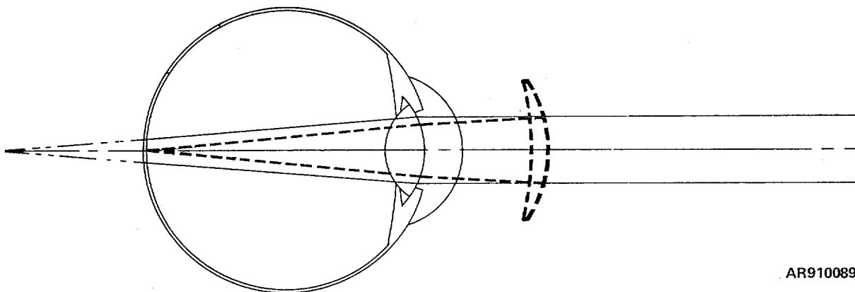
Figure 3-11. Farsightedness (hypermetropia)
