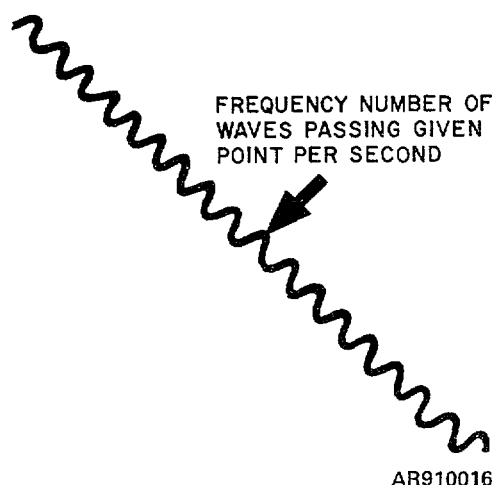
Figure 2-10. Frequency
