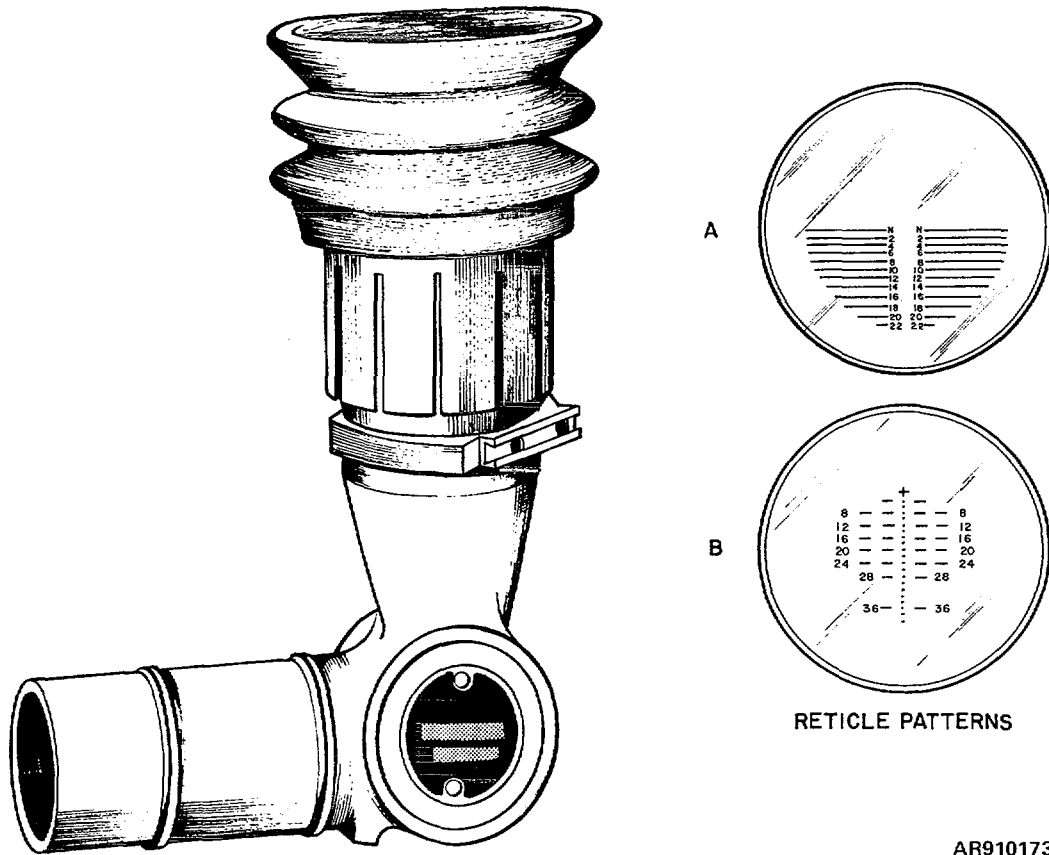
Figure 8-9. Elbow telescope (Howitzer)- assembled view, reticle patterns.
