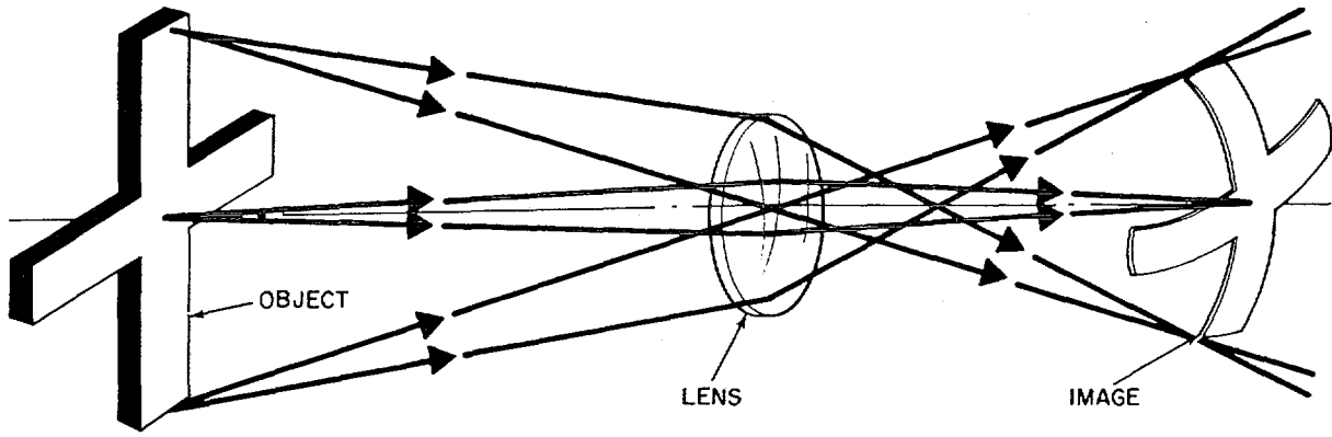
A - CURVATURE OF REAL IMAGE
