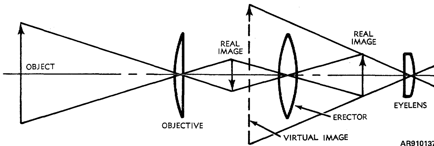
Figure 5-9. Terrestrial telescope—simple form.
