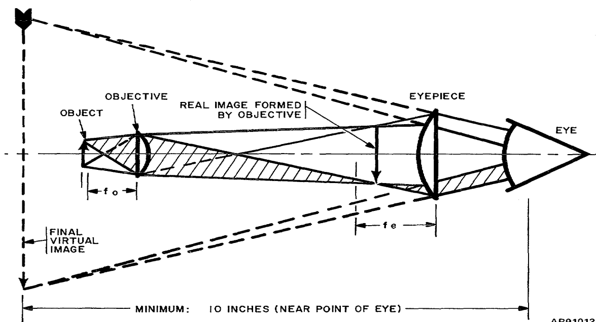
Figure 5-3. Simple compound microscope
