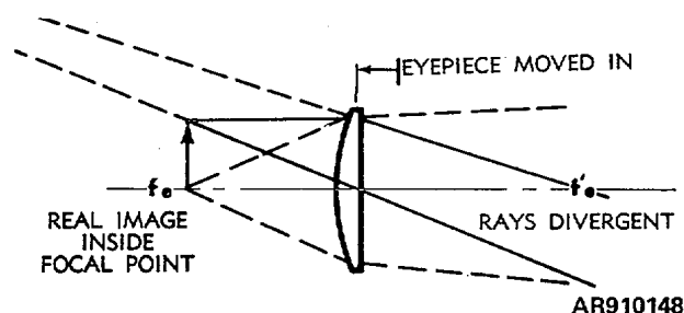
Figure 5-20. Minus setting for shortsighted eye
