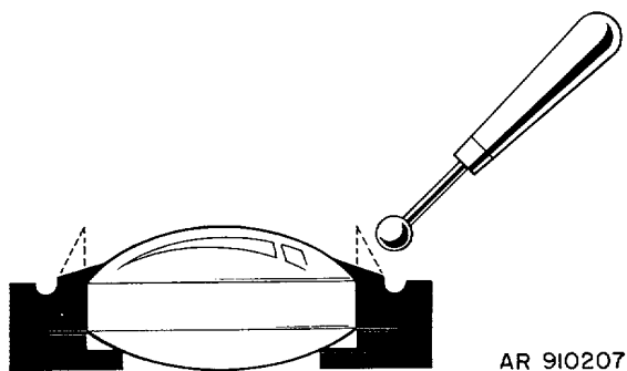
Figure B-7. Burnishing
