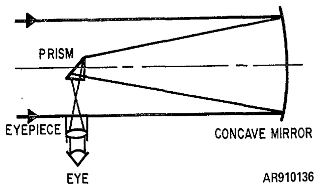
Figure 5-8. Reflecting astronomical telescope.
