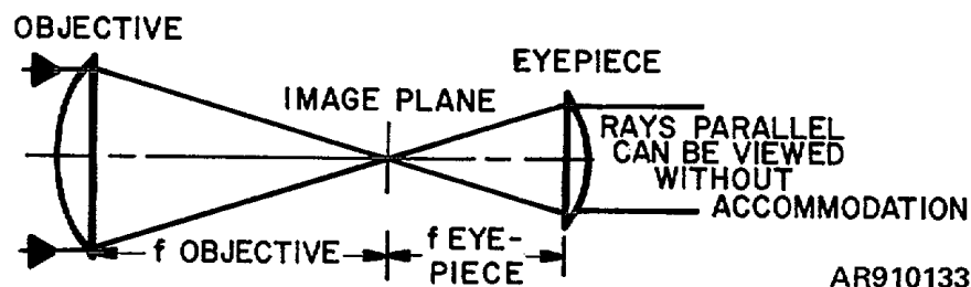
Figure 5-4. Objective lens.
