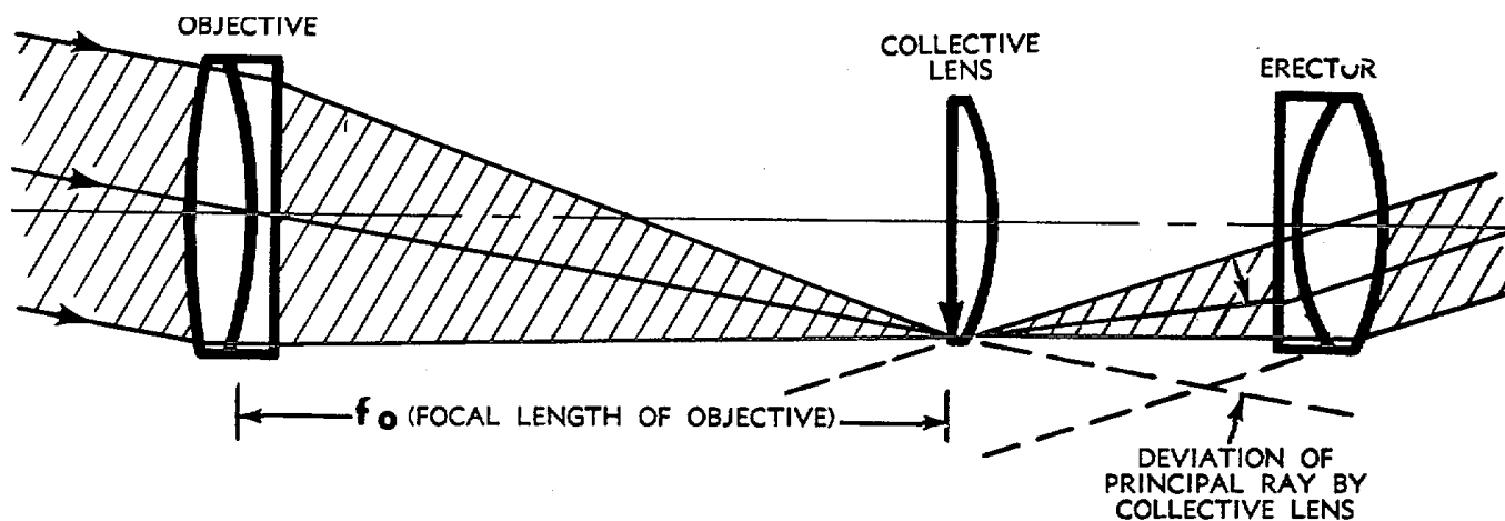
Figure 5-16. Function of collective lens.
