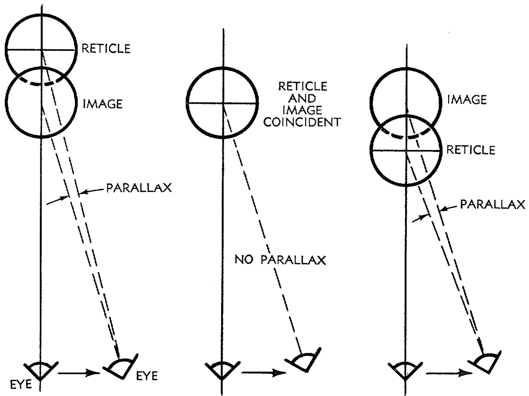
B—PARALLAX IN TELESCOPIC SIGHT
