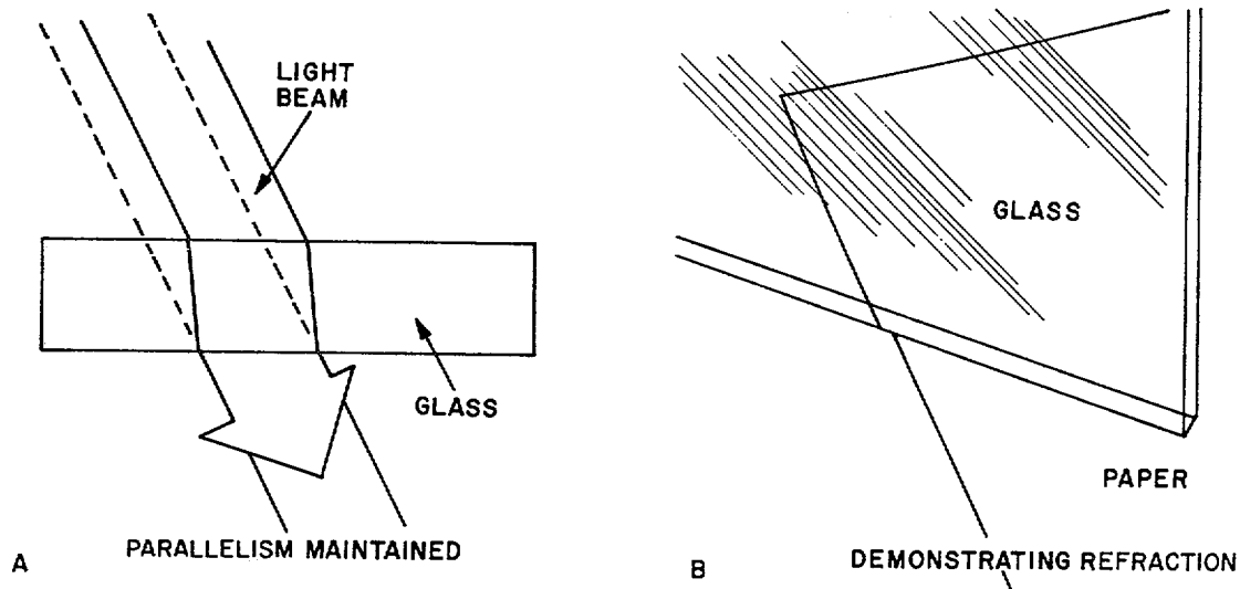
Figure 2-23. Effects of refraction.
